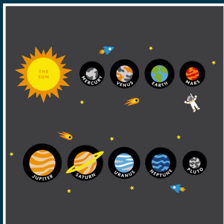
Solar System
