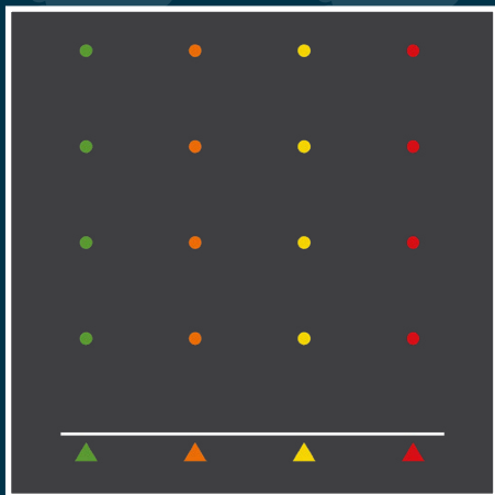
Shuttle Runs
